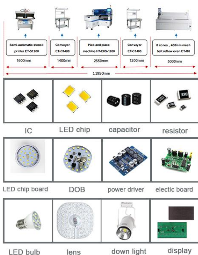
ETON - HT-E8S-1200 Semi-automatic Production Line
