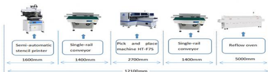
ETON HT-F7S Semi-automatic Production Line
