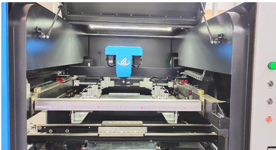
Automatic stencil printer machine main part picture
