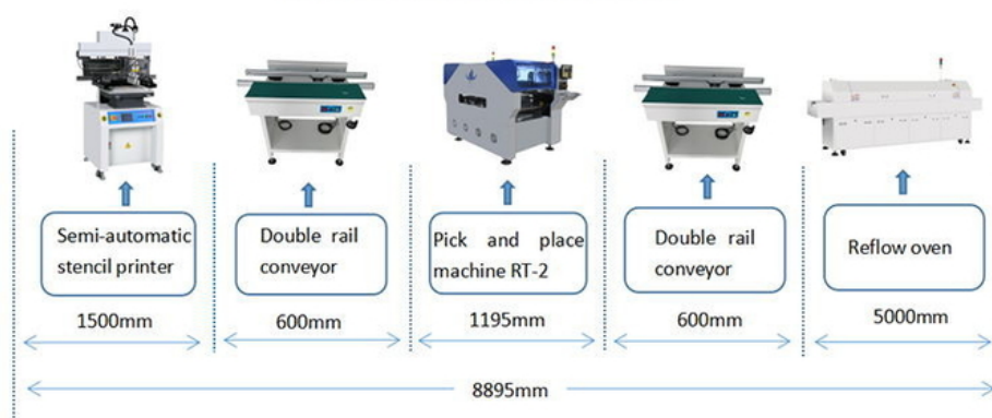
ETON RT-2 Semi-automatic Production Line
