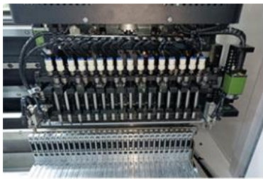
Mounting head
