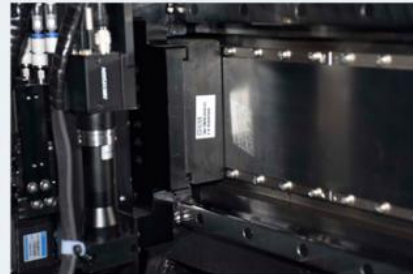
▲ X,Y,Z DRIVE WAY Magnetic linear motor Servo motor
